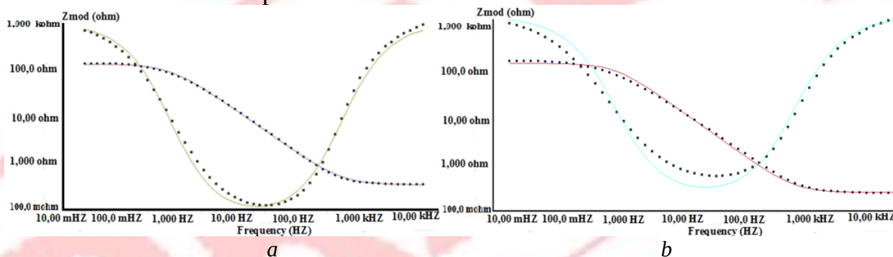
Fig.1. a Bode diagram: a) sample 1. Agreement of model spectrum (solid line) with the experimental data. The extent of congruence 2,44 \cdot 10^{-3} . b) sample 2. The extent of congruence 1,35 \cdot 10^{-3} .
