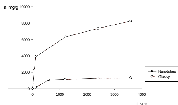
Fig. 1. Kinetic curves formaldehyde adsorption from aqueous solutions with the concentration of 5,85-7,07 mol/l in the presence of phosphoric acid by a carbon porous materials at 75 °C.
