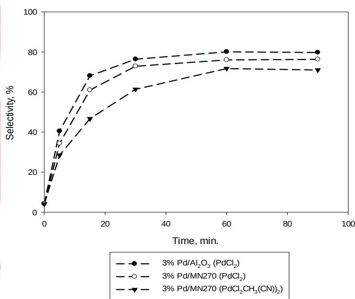
Fig. 1. The dependence of the selectivity for furfuryl alcohol from time to time in the presence of different palladium catalysts
