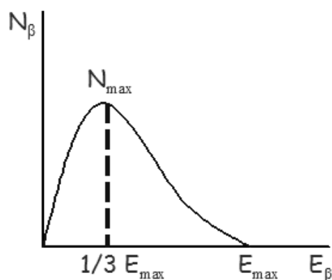
Fig. 1. Spectrum of \beta -radiation.
